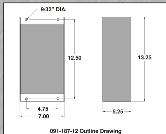
091-187-12 Outline Drawing
