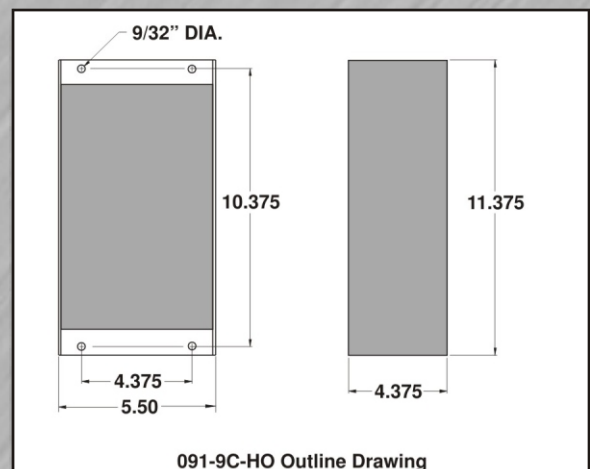
091-9C-HO Outline Drawing
