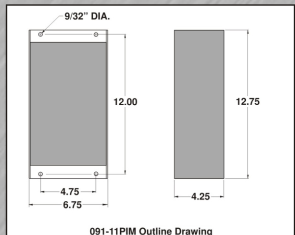
091-11PIM Outline Drawing
