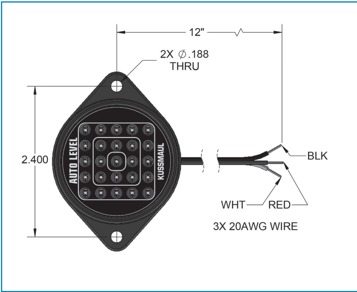
Outline Drawing
